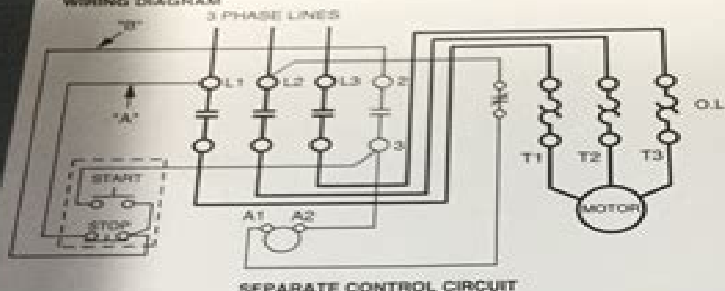
SEPARATE CONTROL CIRCUIT
