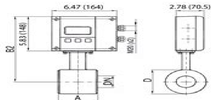
Process Connection Wafer Mounted Version in. (mm)
