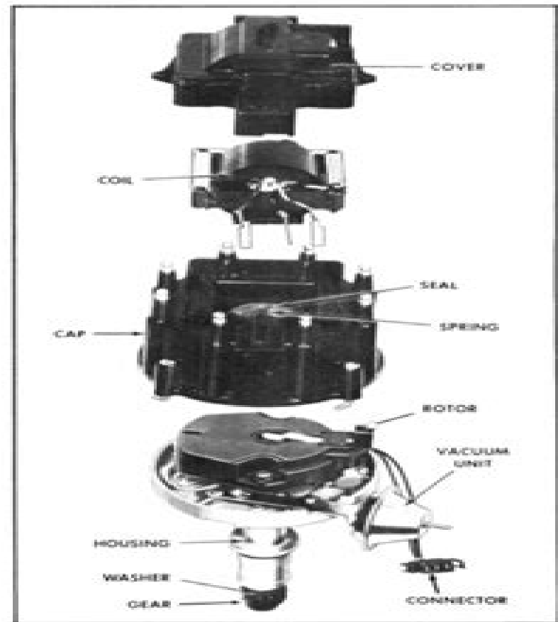
Fig. 10i—Exploded View of 8 Cylinder HEI Distributor
