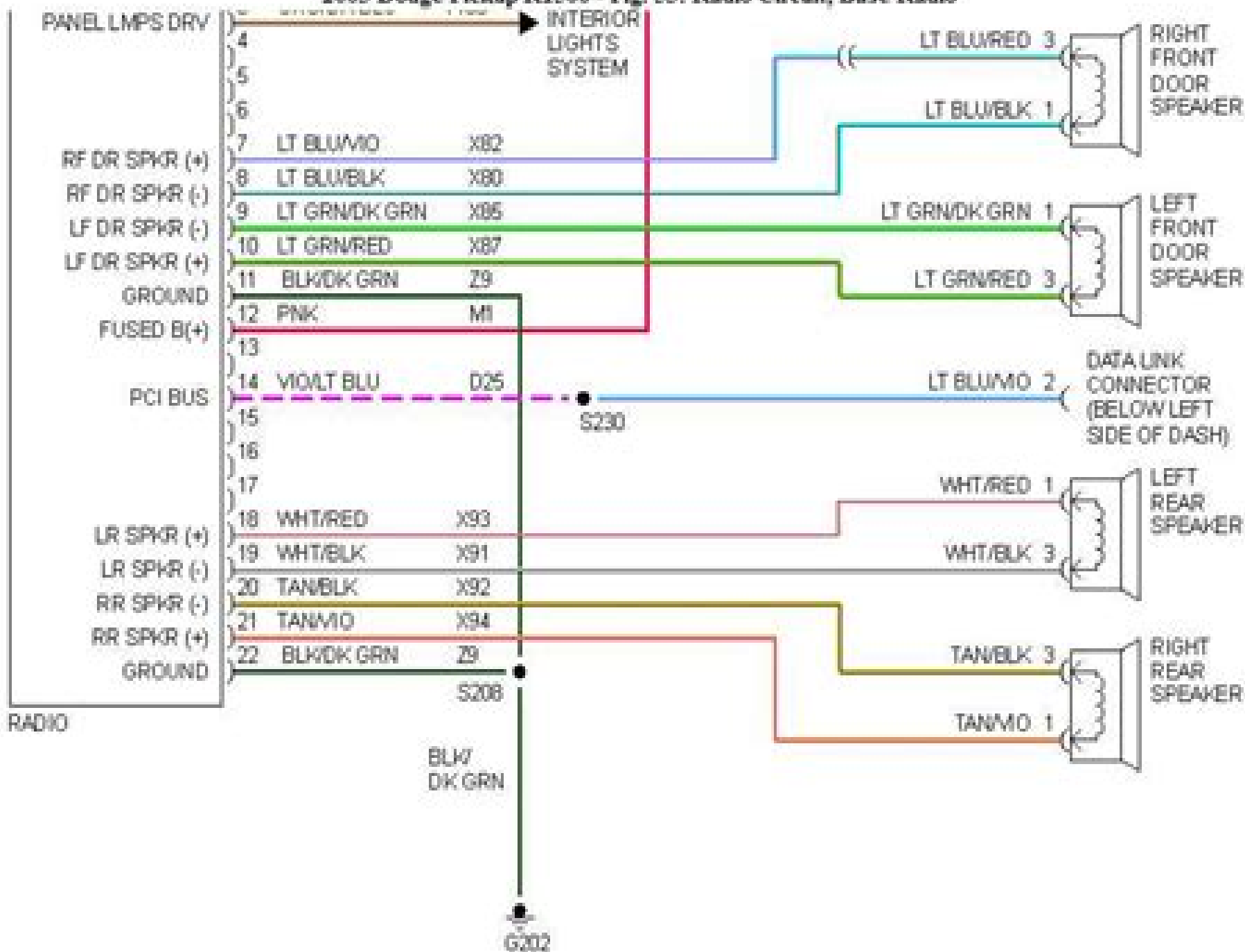
2003 Dodge Pickup R1500 - Fig. 53: Radio Circuit, Base Radio
