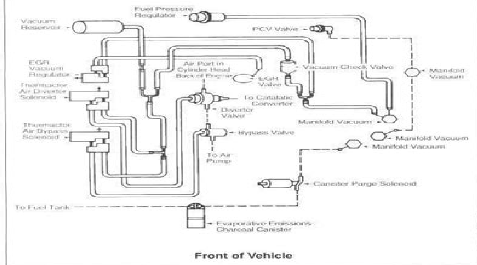
Figure 24 VACUUM HOSE ROUTING SCHEMATIC (Typical Routing, Similar to 1987- 93 5.0L H.O. Mustang)
