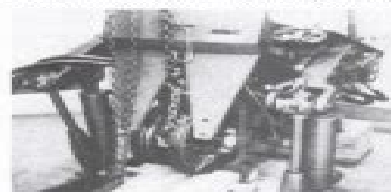
Fig. 262—Use a wood block as protection and roll differential assembly rearward out of center housing.
