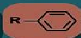
ARENE
