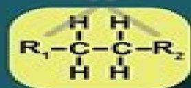
ALKANE
