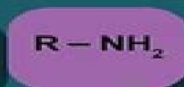
AMINE
