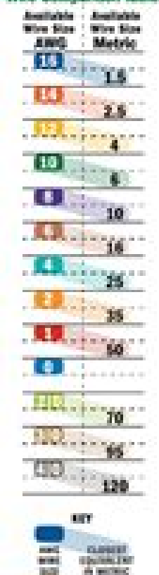
Standard and Metric Wire Comparison Table
