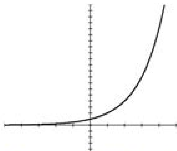
Exponential Growth
