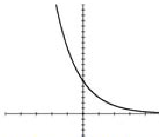
Exponential Decay
