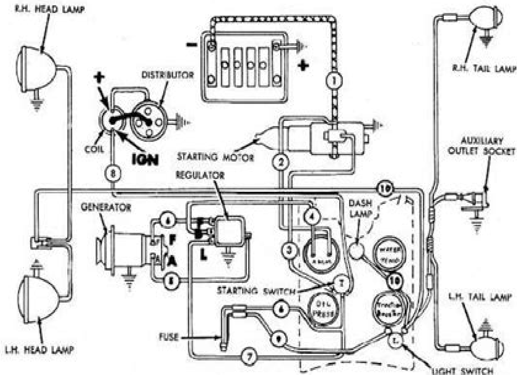
Fig. 185—Wiring diagram for D-15 non-diesel tractors. The twelve volt battery has positive (+) terminal grounded. Refer to Fig. 184 for color code.
