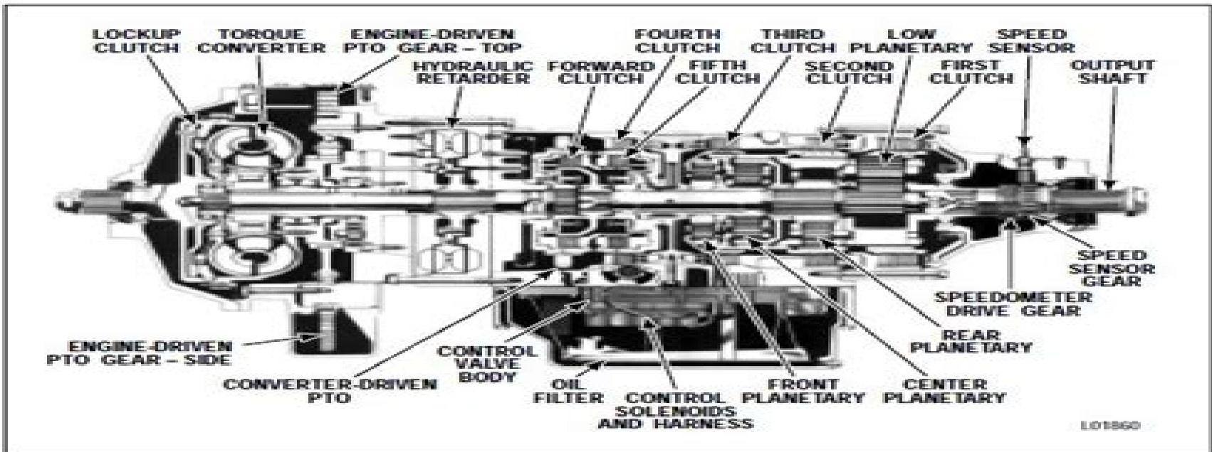
Cross Section of CLBT 755
