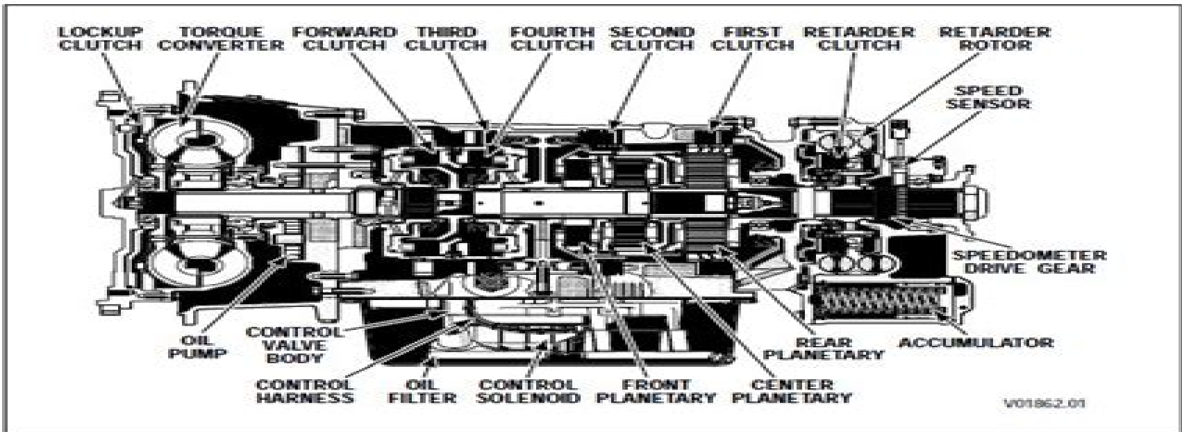
Cross Section of HTB 748
