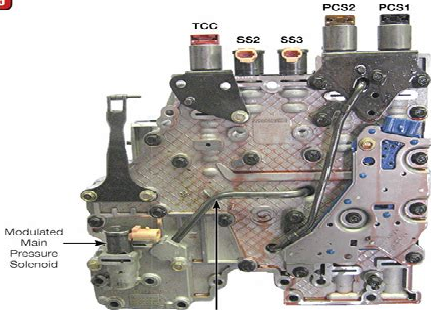
Additional tube identifies the '06-'09 Allison 6-speed.
