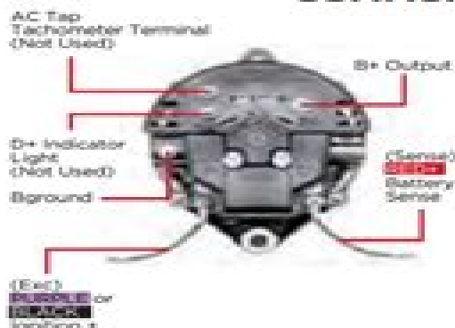
LATE MOTOROLA/PRESTOLITE STYLE FITS MERCURISER & OMC
