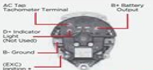
LATE MOTOROLA/PRESTOLITE STYLE FITS U.S. MARINE
