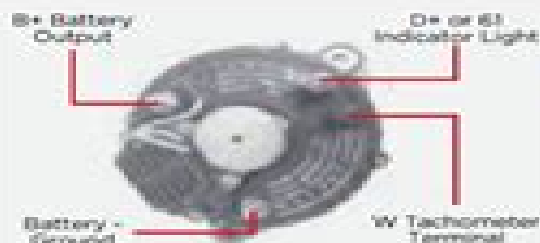
VALEO/PARIS RHONE FITS VOLVO PENTA
