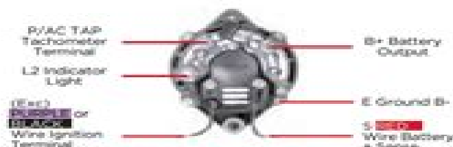
LATE MANDO STYLE FITS MERCURISER AND OTHERS
