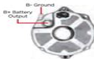
DELCO SELF EXCITING STYLE FITS MERCURISER AND OMC
