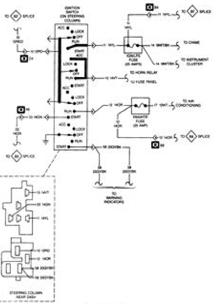
IGNITION SWITCH
