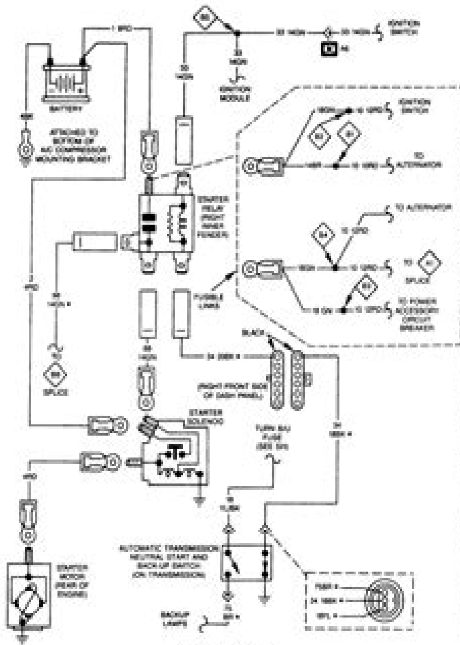
STARTER SYSTEM
