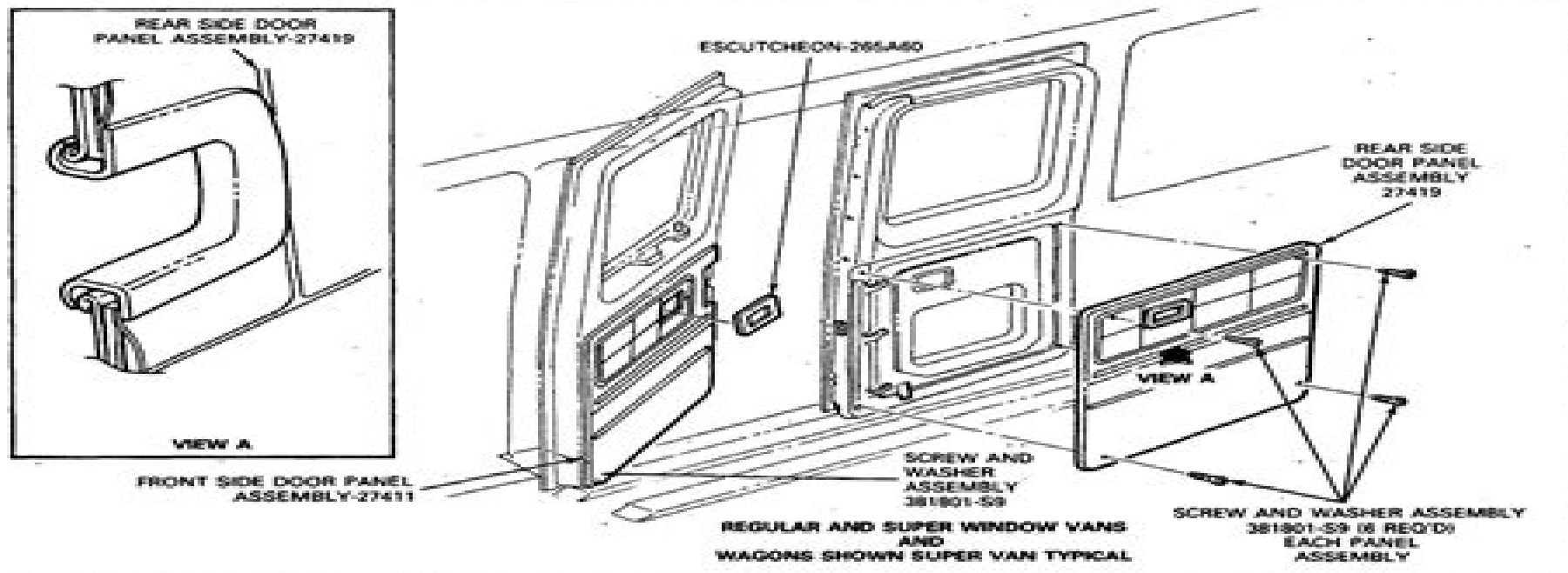
FIG. 8 Side Hinged Door Trim Panel—E-150—E-350
