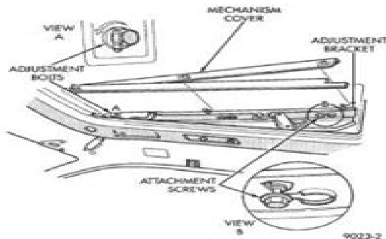
Fig. 3 Glass Height Vertical Adjustment
