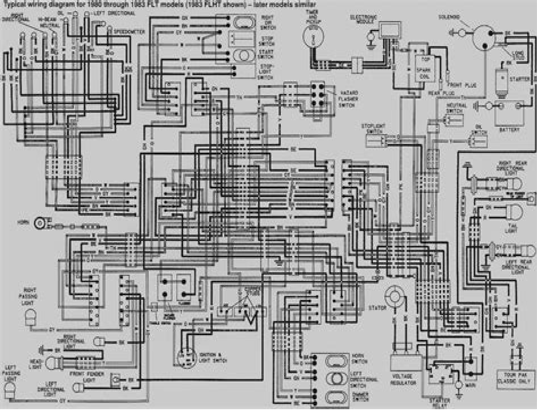
Typical wiring diagram for 1980 through 1983 FLT models (1983 FLHT shown) - later models similar
