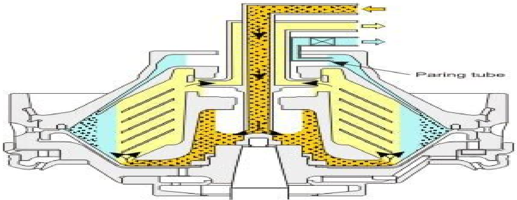
S-separator bowl
