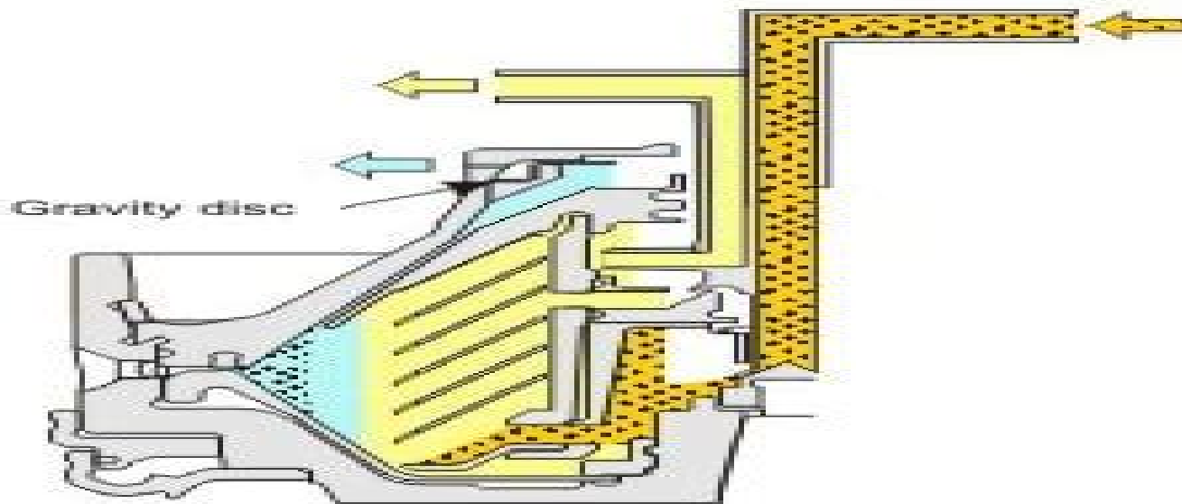
P-separator bowl
