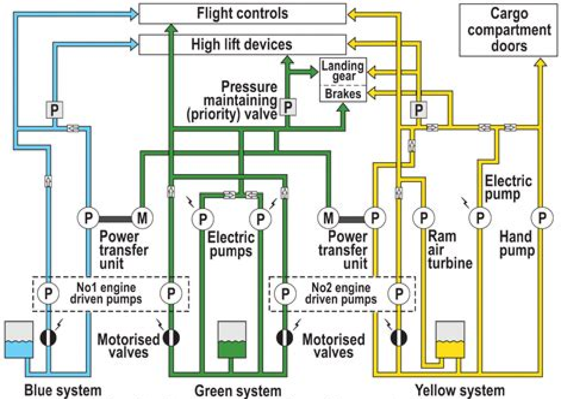
Typical twin engine hydraulic system layout
