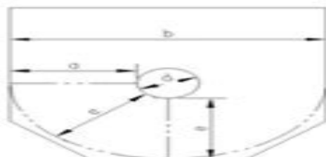
AISC Preferred Geometry
