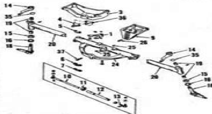
Fig. 4-Heavy duty adjustable wide front axle available for all Farmall tractors.
