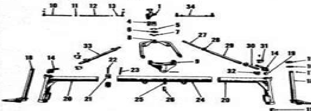
Fig. 6-Expanded view of adjustable wide front axle used on Farmall "Hi-Clear" models. Note the auxiliary stay rod assemblies.
