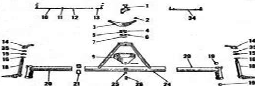
Fig. 4-Heavy duty adjustable wide front axle available for all Farmall tractors.
