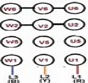
STAR CONNECTION
