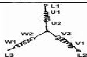
(1) STAR CONNECTION ( 6 LEADS)
