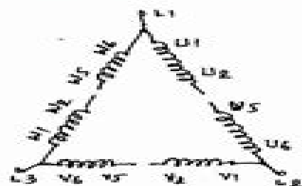
(3) DUAL VOLTAGE(STAR STARTING & DELTA RUNNING) (12 LEADS)
