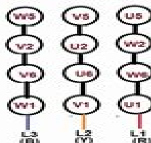
DELTA CONNECTION
