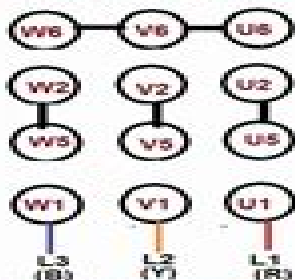
LOW VOLTAGE CONNECTION
