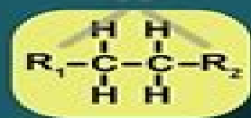
ALKANE
