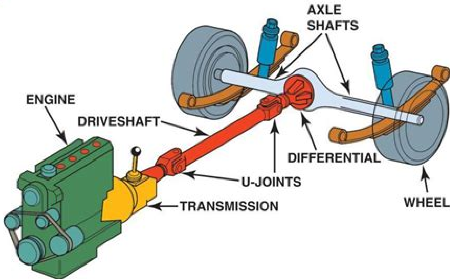
FIGURE 38.15 Typical rear-wheel-drive power train arrangement. The engine is mounted longitudinal (lengthwise).
