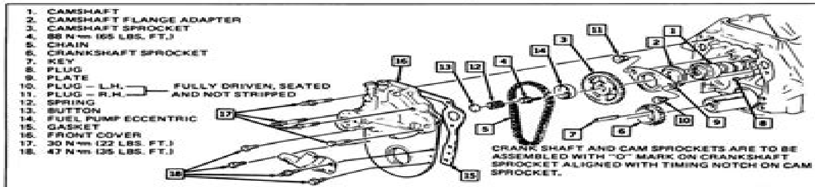
Fig. 32 Front of Engine
