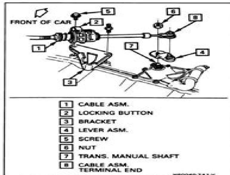
Figure 7A1-5 Shift Control - Cable Adjustment
