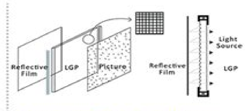
Engraving and Scribing Diagram
