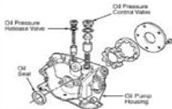
Fig. 26. Exploded View Of Oil Pump & Components Courtesy of GENERAL MOTORS CORP.
