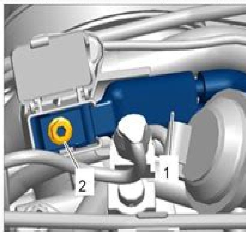
Fig 1: Identifying B+ Line Connection Point With Hexagon Nut (Engine Compartment)
