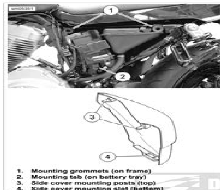
Figure 2-160. Left Side Cover: XR Models
