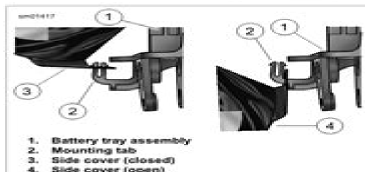
Figure 2-161. Left Side Cover Bottom Mount: All Models
