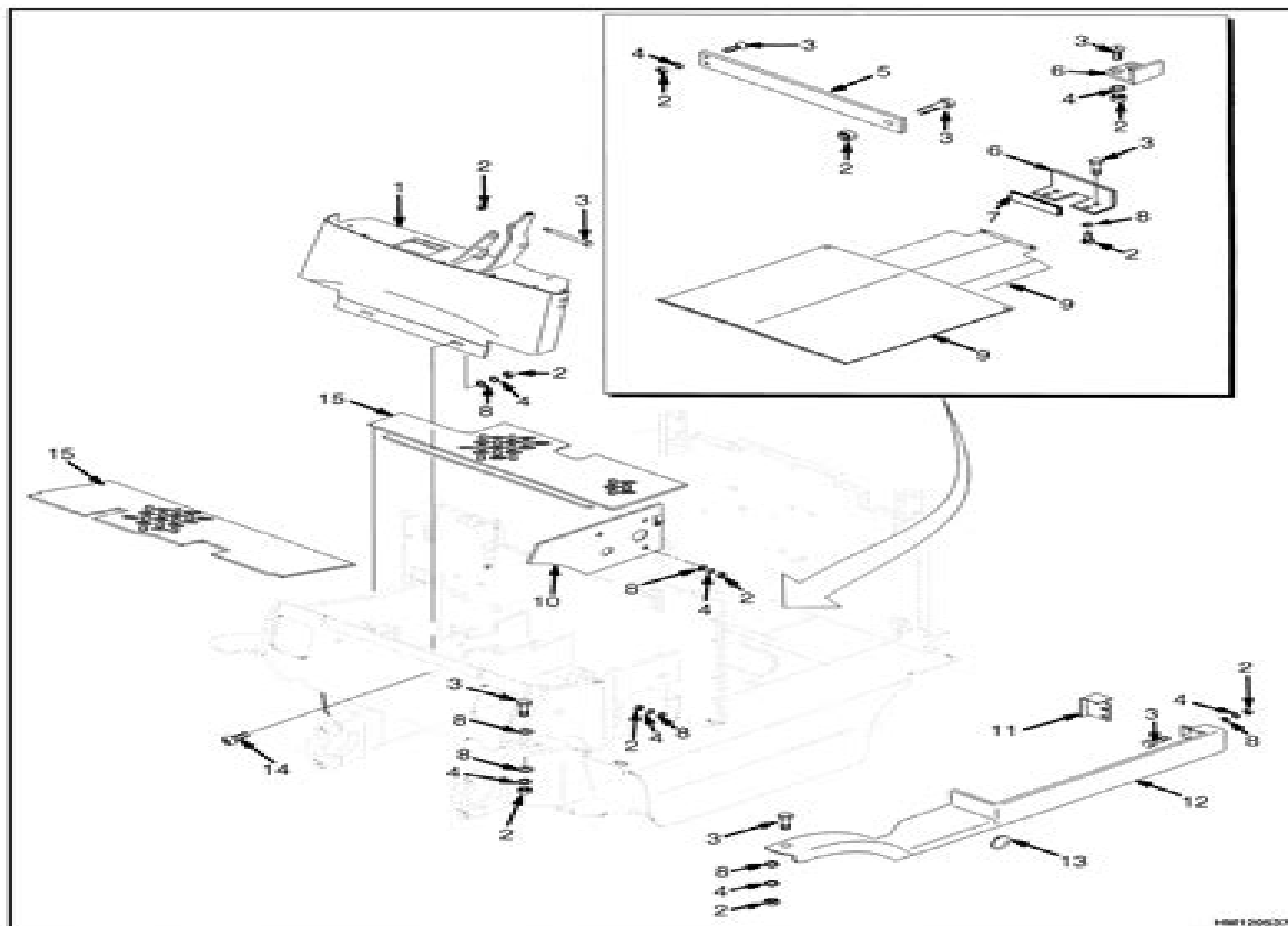
Figure 2. Lift Truck Frame Manual Hydraulics ERC/P16-20AAF (ERC030, 040AH) (C814)
