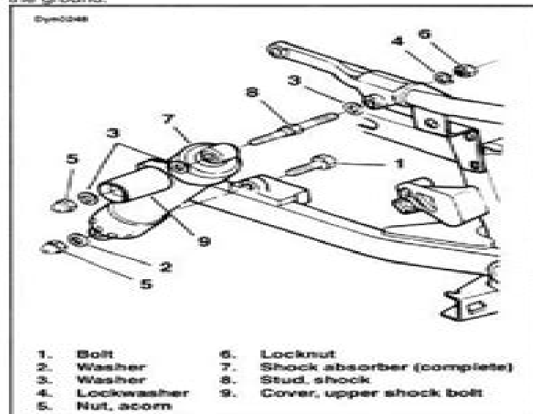
Figure 2-62. Rear Shock Absorber Mounting
