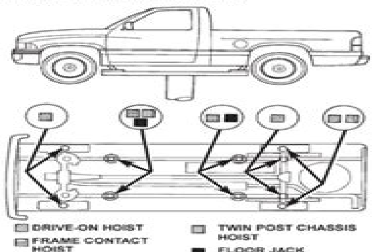
Fig. 7 Correct Vehicle Lifting Locations—Typical
