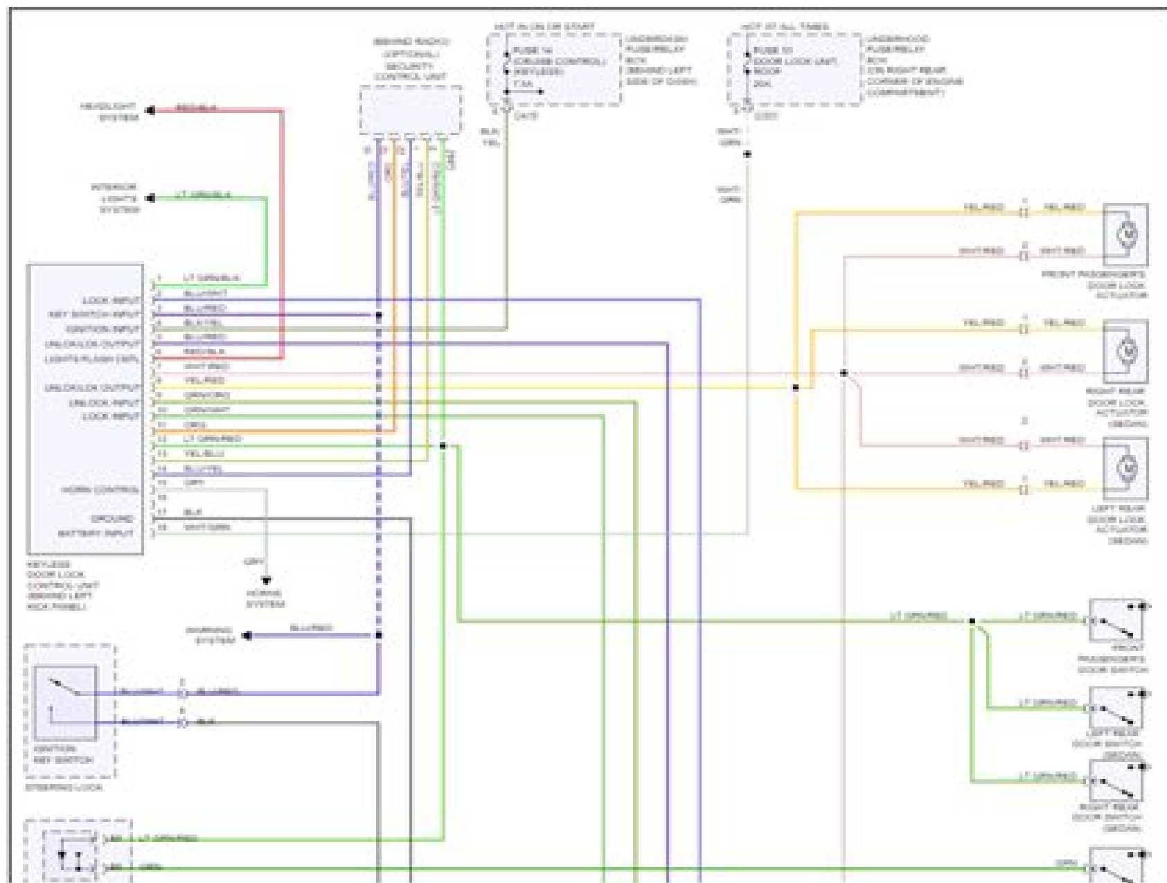
Fig 1: Power Door Lock Circuit, W/ Keyless Entry
