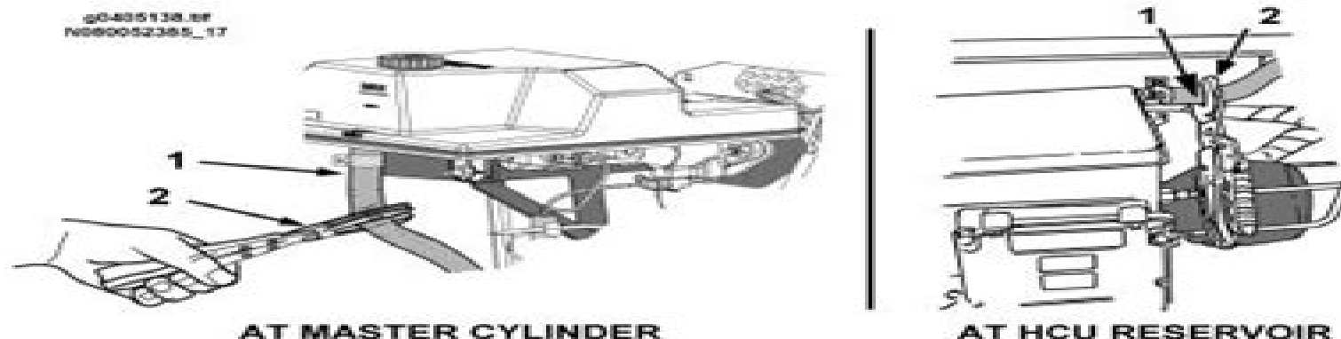
Figure 38 Clamping the Low Pressure Hose
