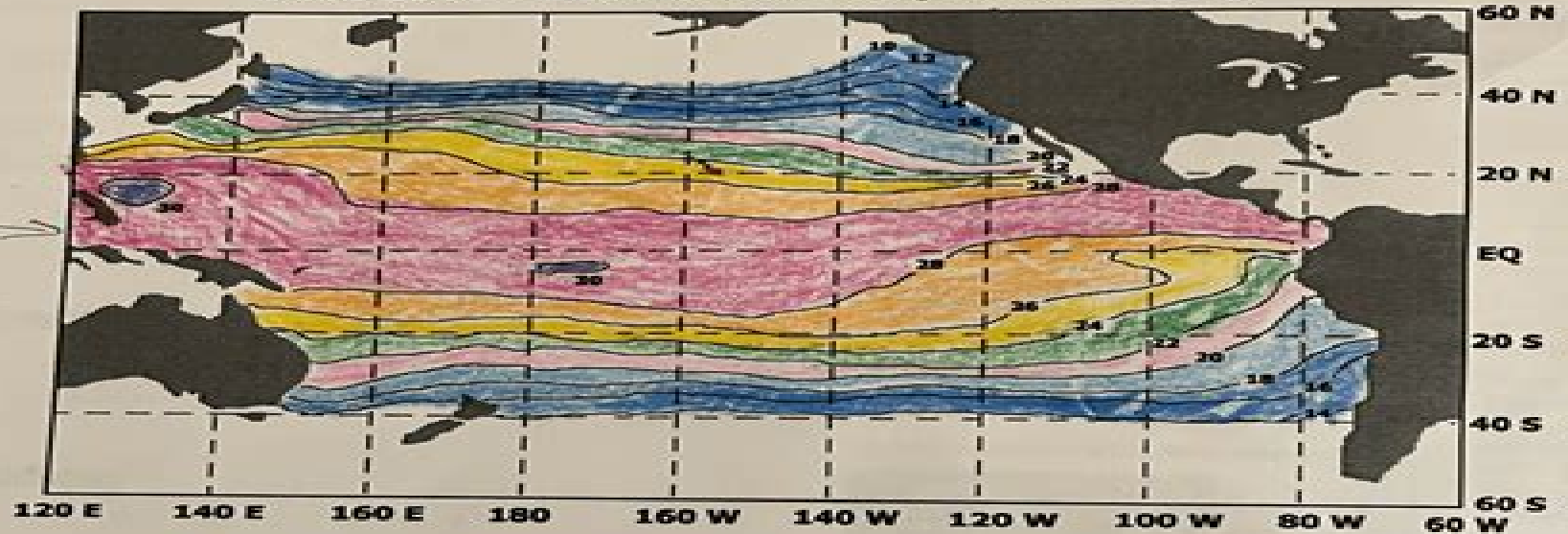
June 1988 - Sea Surface Temperatures (C°)
