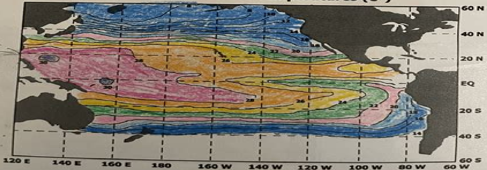
June 1988 - Sea Surface Temperatures (C°)
