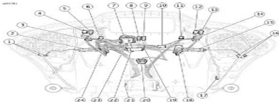
Figure 1. Handlebar, FLH Fairing Models
