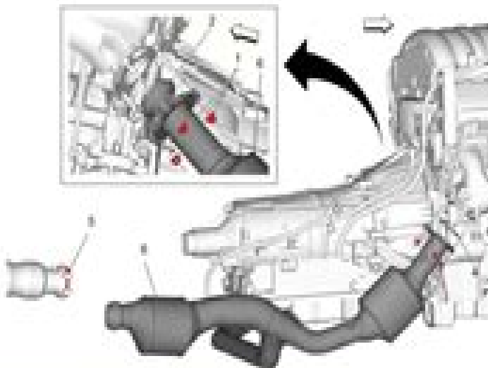
Fig. 283: Three-Way Catalytic Converter (L31, L33, L43, or L46)
