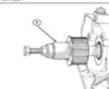
Fig. 42 Crankshaft Sprocket - Installation 1 - SPECIAL TOOL 8792
