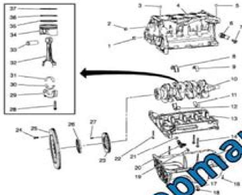
Fig. 7 Identifying Engine Block Assembly Components
