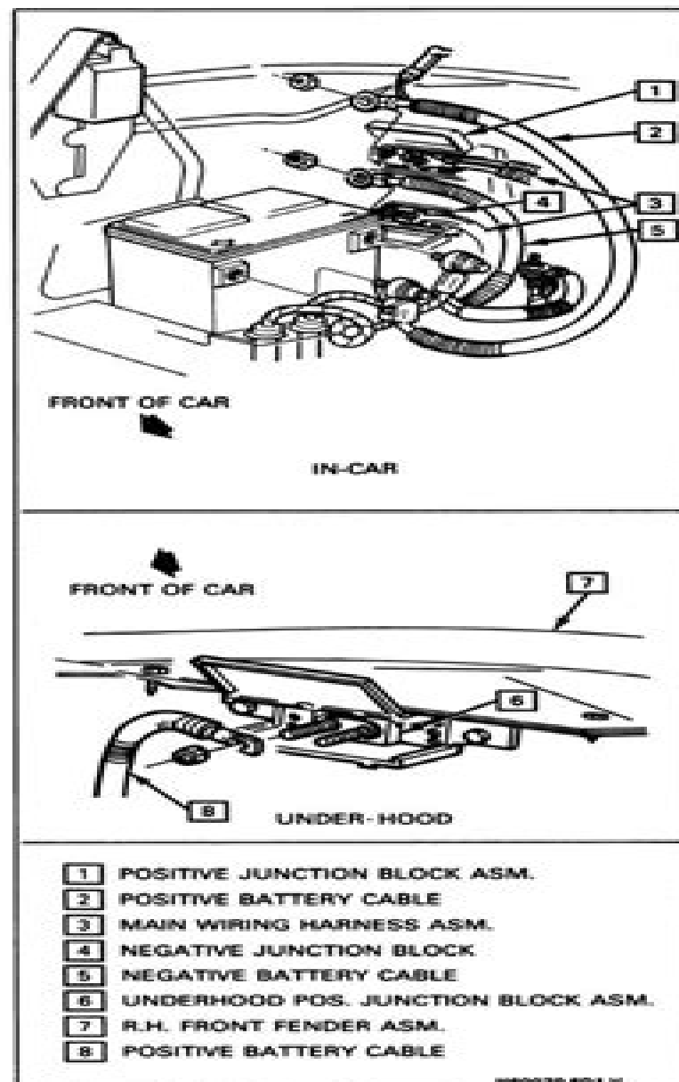
Figure 6D1-7 Battery Cables at Junction Blocks
