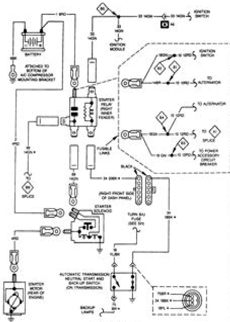
STARTER SYSTEM
