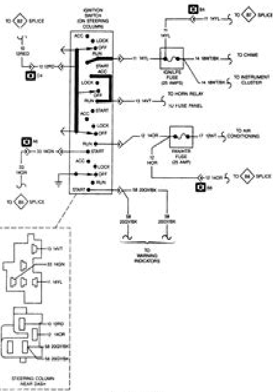
IGNITION SWITCH
