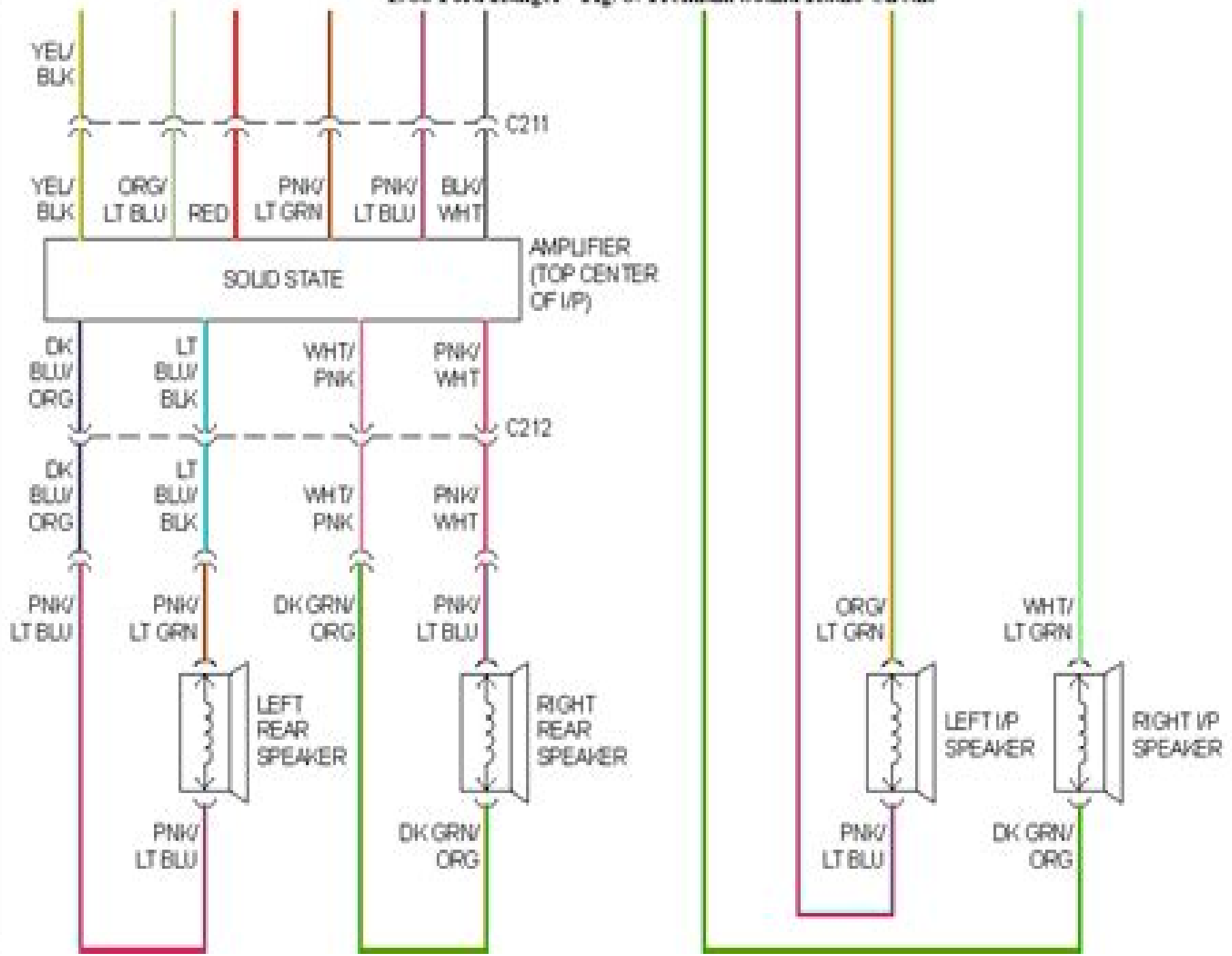
1988 Ford Ranger - Fig. 8: Premium Sound Radio Circuit
