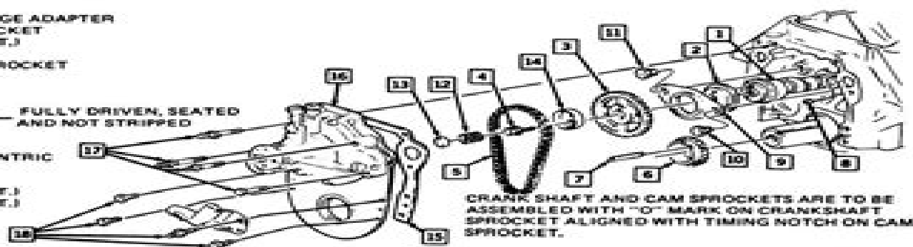
Fig. 32 Front of Engine
