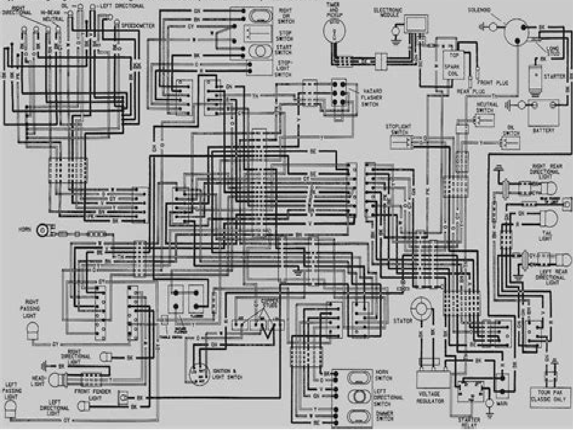
Typical wiring diagram for 1980 through 1983 FLT models (1983 FLHT shown) - later models similar
