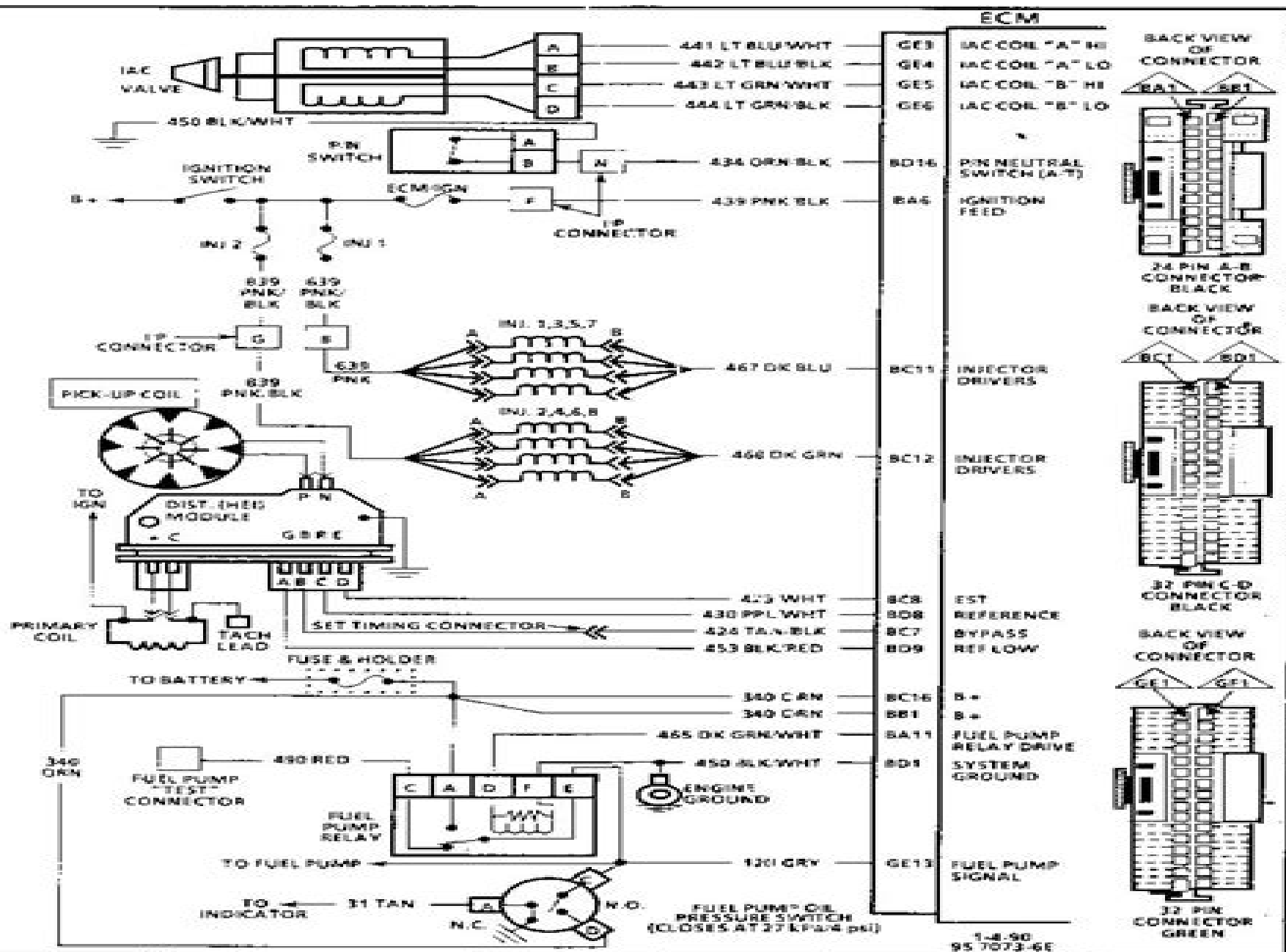
Figure A-3 - ECM Wiring Diagram 5.0L (VIN F) &amp; 5.7L (VIN 8) "F" Carline (2 of 4)
