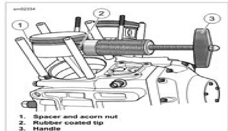
Figure 3-29. Piston Pin Remover (Part No. HD-42320-A)
