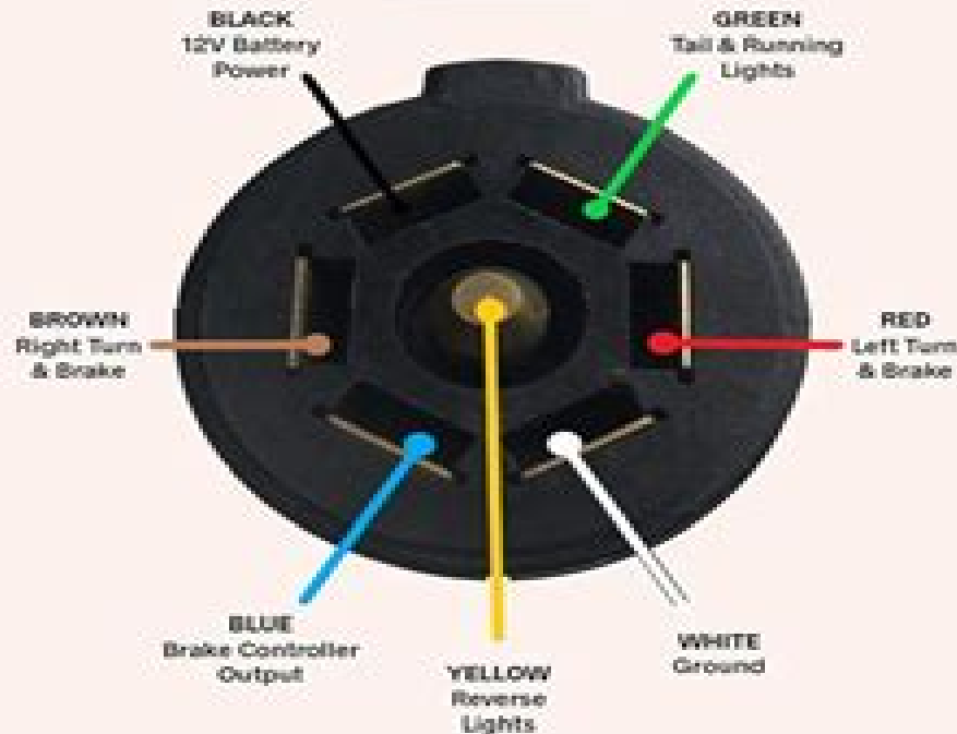
Plug Side
