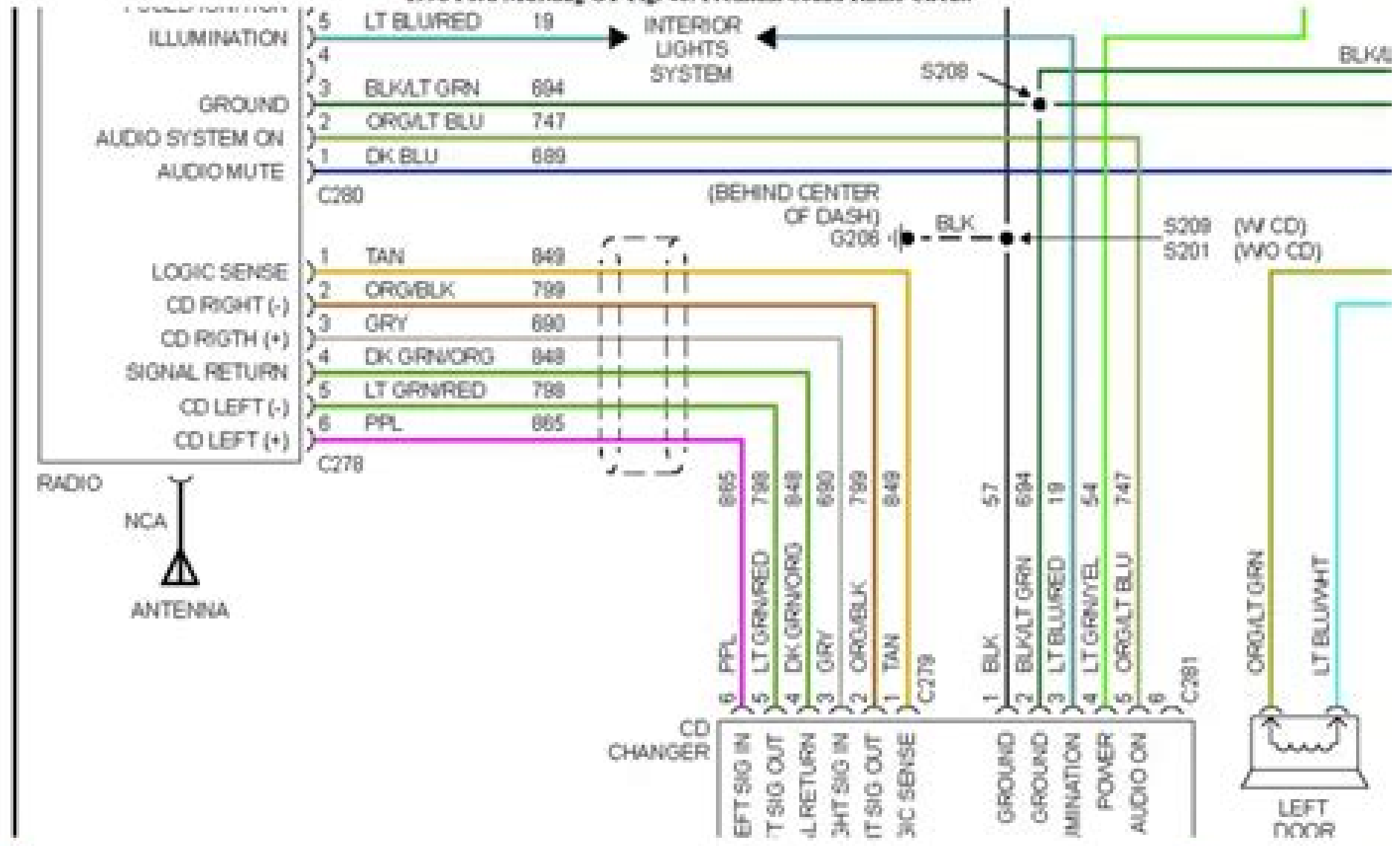
1998 Ford Mustang GT-Fig. 46: Premium Sound Radio Circuit
