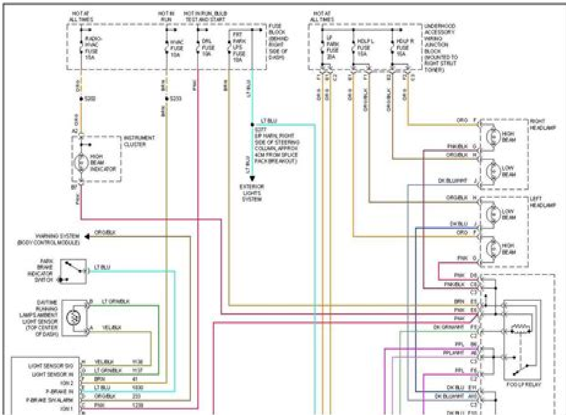
1998 Buick Regal GS—Fig. 29: Headlight Circuit
